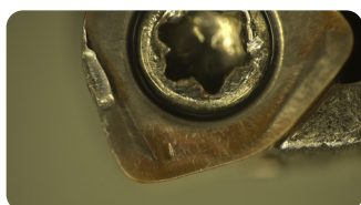
Tool wear after 30 minutes of machining
