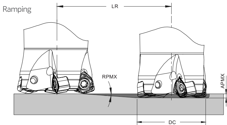
Helical Interpolation
